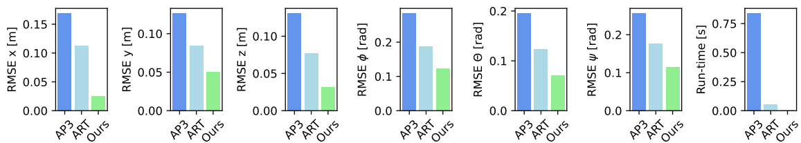
Figure 9. A summary statistics. Root Mean Squared Error (RMSE) and run-time are reported for the baseline methods and the proposed extension to the ARTOOLKITPLUS. Lower the better for both the measures.
