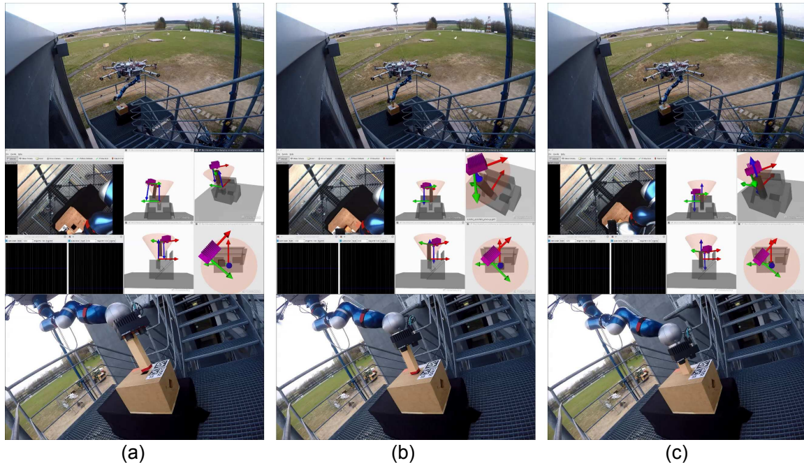
Figure 16. Qualitative results for peg-in-hole task with the aerial manipulator. (a) Approach phase, (b) precise positioning, and (c) successful insertion. Top: overview of the robot's remote workspace, where SAM is suspended by a crane. Middle: the operator view with live video streams, and the created VR, which displays four different view points simultaneously, and provides haptic guidance in both position and orientation. Bottom: close view on the robot's workspace. With the proposed VR based system, the operator is able to achieve precise peg-in-hole task with the robot in outdoor environments. The markers of size 2.5 cm ( \times 3 ), 6.25 cm ( \times 1 ), and 10 cm ( \times 1 ) are used in this scenario.
