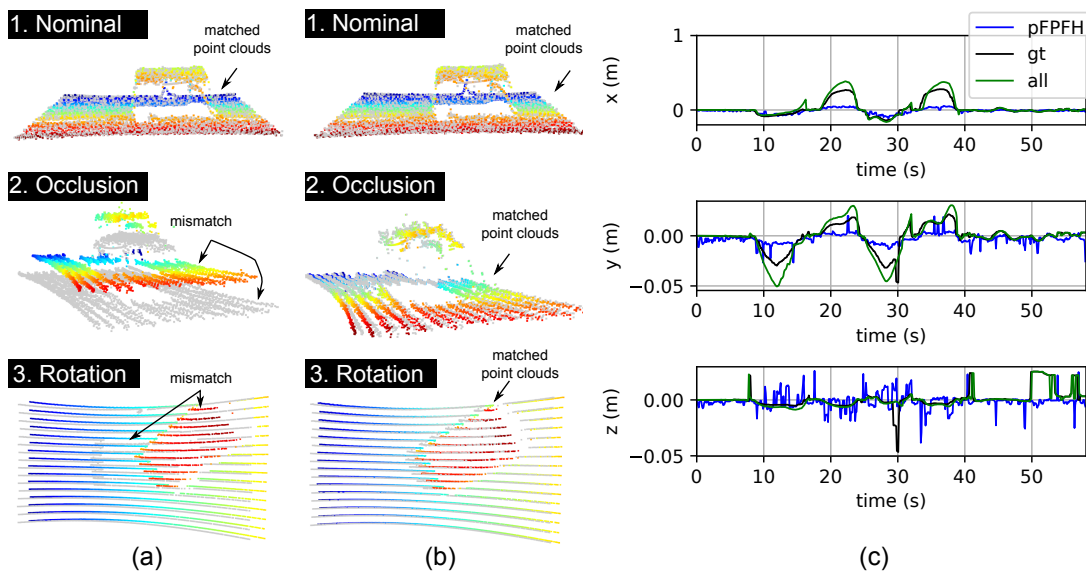
Figure 12. Qualitative results for the LiDAR based object pose estimators. (a) Evaluation of a vanilla object pose estimator. (b) Evaluation of the proposed object pose estimator. (c) Plots of the estimated positions from a baseline (pFOFH) and our approach (all) against the ground truth (gt) measurements. The qualitative results over occlusion and rotation scenarios justify the design choices of the proposed method. The monotonic gray indicates the source point cloud while the colored point cloud refers to the current scan. All point clouds are cropped for the visualization purpose.
