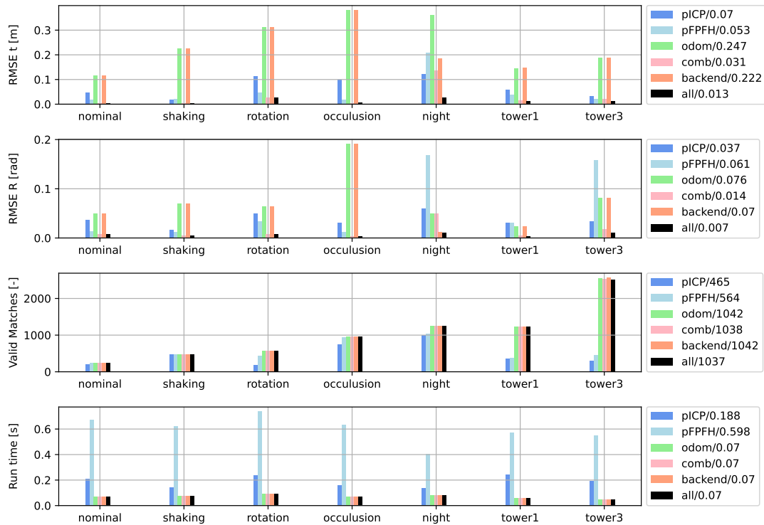
Figure 11. Statistical analysis of the baselines and the proposed method per scenario. Lower the better for the RMSE and run-time, and higher the better for the number of valid point cloud matches. These results indicate that the proposed algorithm can cope with the identified challenges, thereby justifying the design choices of the algorithm.
