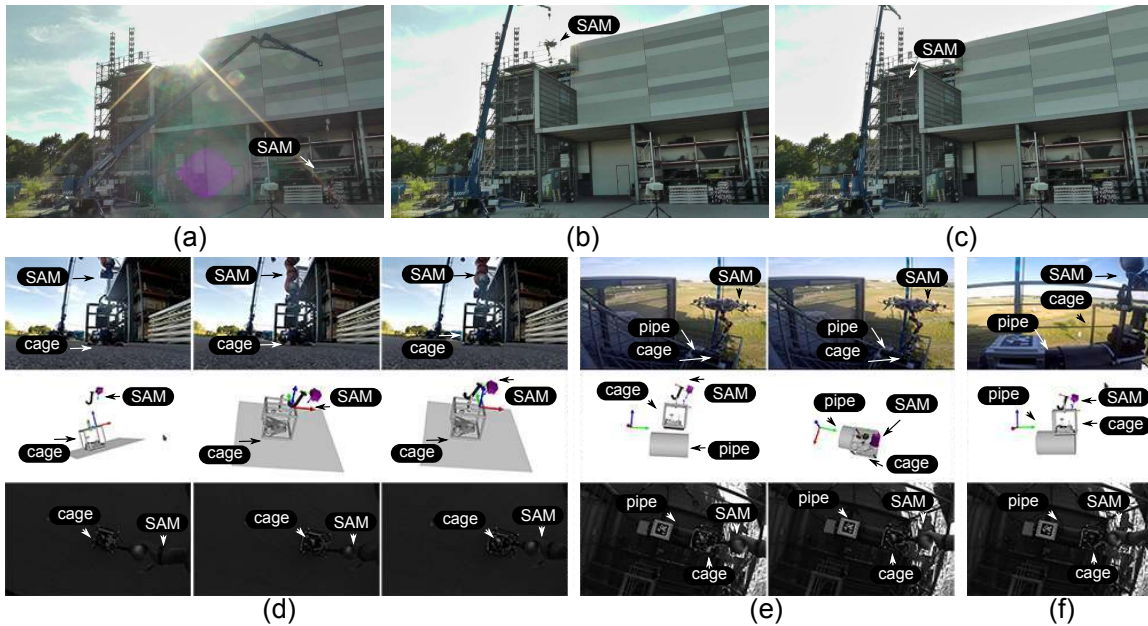
Figure 17. Qualitative results for deployment of robotic crawler within an industrial inspection and maintenance scenario. [(a)–(c)] The carrier brings the robot from the ground to the remote location. (d) The robot picks the cage that carries the inspection robotic crawler. (e) The robot places the cage on a mock up of an industrial pipe. (f) The robot exerts force on the cage, so that the crawler can roll out of the cage without falling. The operator can use the VR (bottom), which contains 3D information as opposed to 2D camera images (middle). Live video stream is also subject to over and under exposure when under a shadow on a bright day. With the proposed VR based system, the robot is able to execute advanced aerial manipulation tasks for the considered real world application. Four markers of size 5cm are used for the cage hosting the mobile robot. The first experiment used a marker of 25 cm on the pipe with its CAD model. Later these primitives were replaced by the proposed LiDAR based pose estimation algorithm.
