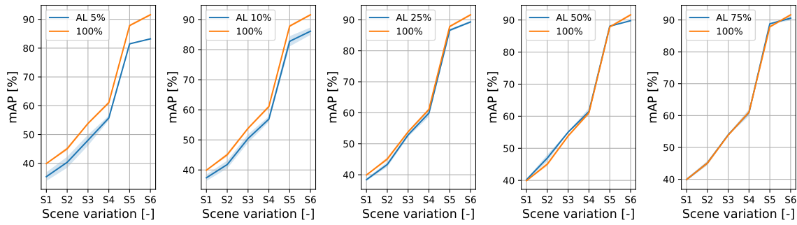
Figure 14. Results of active learning (AL) compared to the training setup that uses 100% of all data over different scenes. AL is used for the acquisition sequence of 5%, 10%, 25%, 50%, and 75% of all data. Higher the better for mAP. The results show that one can save upto 75% of data, in order to reach more than 95% of the total performance.
