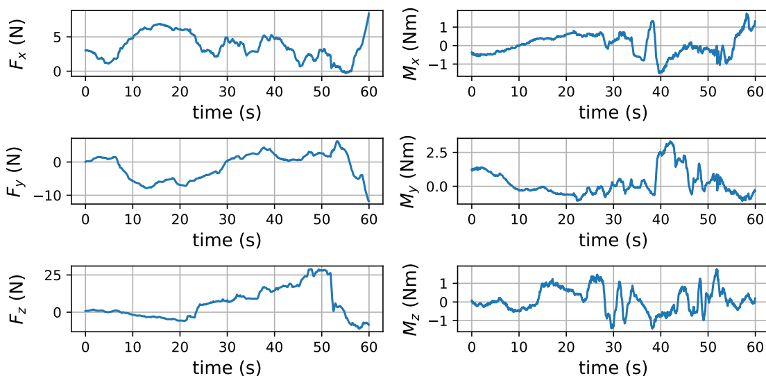
Figure 23. Wrench forces and moments from the peg-in-hole experiments. The poses of the end-effector are alternatively depicted in Figure 19. In F_z , between 50 and 60 s, a drop in force is observed due to the successful peg-in-hole insertion.
