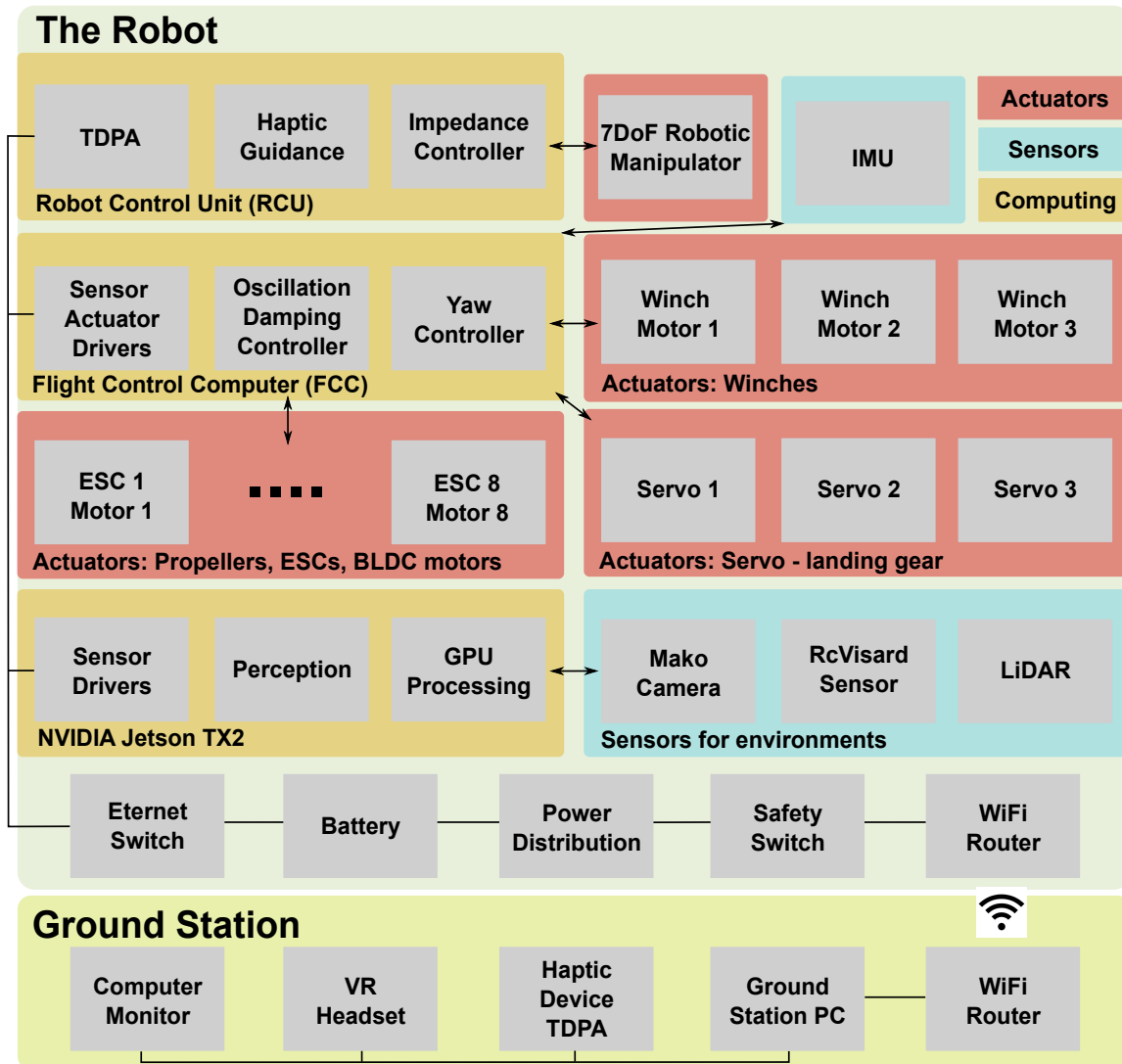
Figure 25. SAM's IT architecture. The broad division is between the ground station and the robot. The ground station hosts haptic device, VR, and the human operator. WiFi routers are used to communicate to the robot, which simulates the real teleoperation scenarios with imperfect communication and delays. The robot hosts computers, actuators, sensors and other auxiliary components such as power distribution, battery, etc. SAM has three computers. The robot control unit (RCU) deals with the control of robotic manipulator and hosts real-time LINUX as its operating system. The flight control computers (FCC) deals with platform control, including propellers, winches and additional servo motors as landing gear. FCC hosts QNX real-time LINUX system. Lastly, NVIDIA Jetson TX2 is used as a vision processing unit. The TX2 hosts non-real-time LINUX (ubuntu tegra) but has a GPU for deploying the deep learning models.
