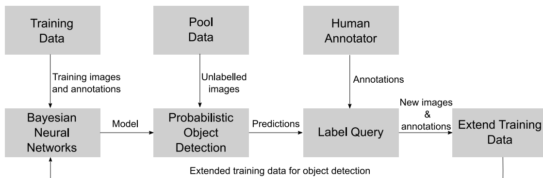
Figure 8. Active learning pipeline for generating labelled data more efficiently. Instead of randomly selecting the images to be labelled, we query the most informative samples from Bayesian Neural Networks - an uncertainty-aware Deep Neural Networks for the state-of-the-art object detection frameworks.
