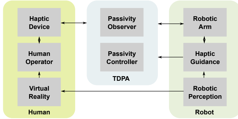
Figure 22. Teleoperation architecture based on Time-Domain Passivity Approach (TDPA). The TDPA approach ensures stability under imperfect communication between the haptic device and the robot and consists of two components, namely, passivity observer and passivity controller. The proposed telepresence system also includes haptic guidance, robotic perception, and VR for 3D visual feedback.
