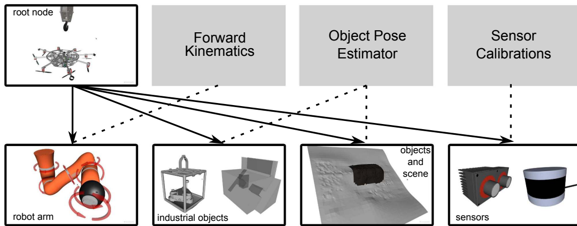
(a) scene graph with flat hierarchy
