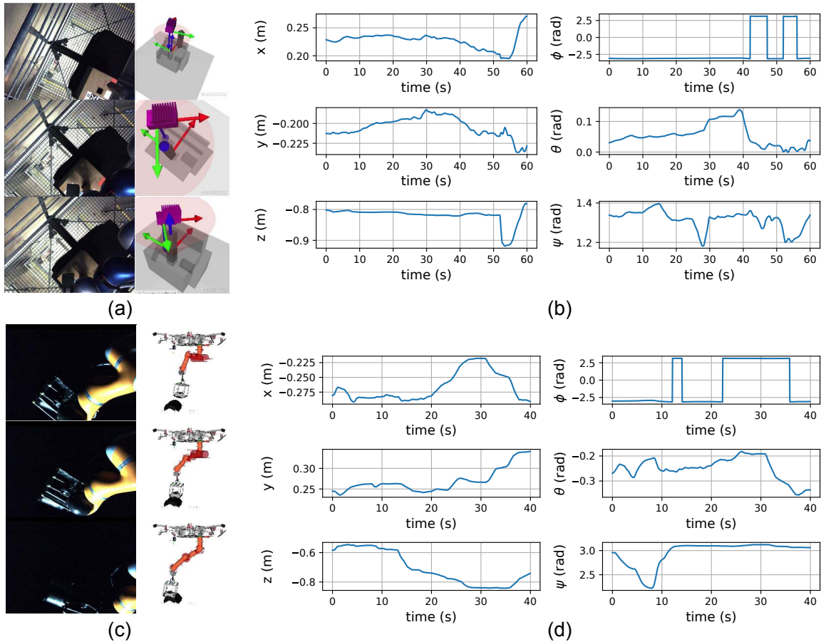
Figure 19. Qualitative visualization of aerial manipulation performed during the night. [(a) and (c)] The camera view and the VR. [(b) and (d)] The translation and the orientation of the robots' end-effector. The corresponding pairs are (a), (b) and (c), (d). These results suggest that the proposed system can extend the operational range of SAM, which further establishes its viability for real world industrial applications. External views are depicted in Figure 20.
