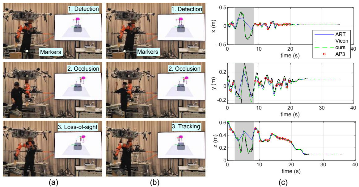
Figure 10. Qualitative results of the proposed marker tracking algorithm. (a) The existing marker tracking algorithms under the loss-of-sight of the markers are evaluated. (b) The proposed extension of the marker tracking algorithm with SLAM estimates is evaluated under the same scenario of the loss-of-sight. (c) The estimated positions from the baselines and the proposed algorithm are compared. These results indicate that the proposed algorithm can cope with the loss-of-sight of the markers and the time delays, thereby justifying the design choices of the algorithm. Three markers of size 2.5 cm, a marker of 6.25 cm, and a marker of 10cm are used in this evaluation scenario.
